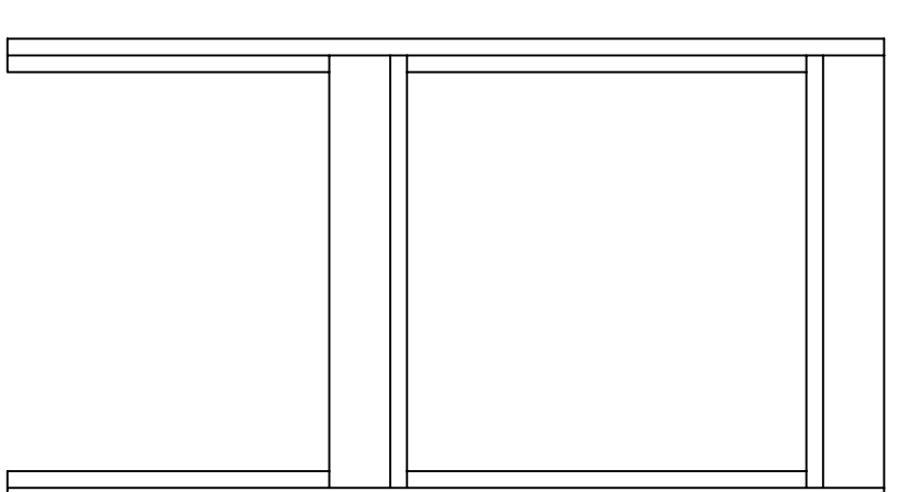
36" x 36" Window Buck 7 - 2x6 x 8'
